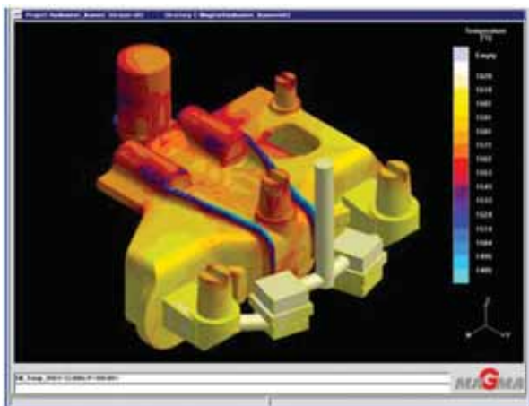
Figure 6 Simulation of temperature distribution
